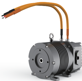
ePower Traction 24V-80V 30KW
